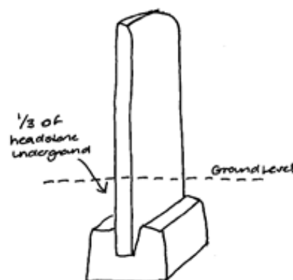
Monolith fixing
